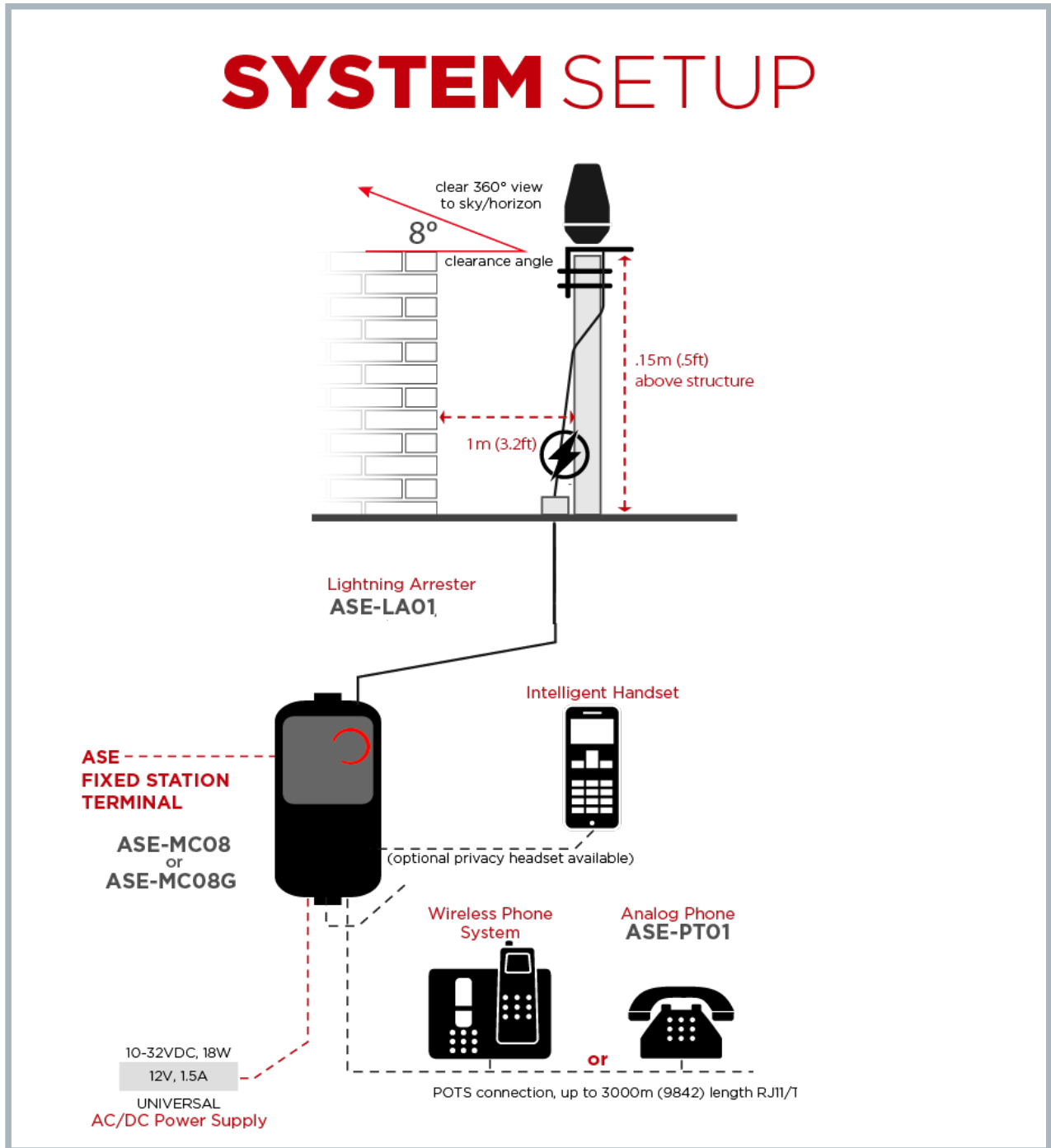
MC08 INSTALLATION DIAGRAM
